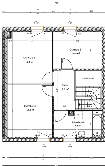
PLAN R+1
